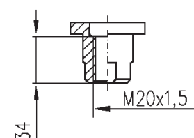
Detail of coupling
